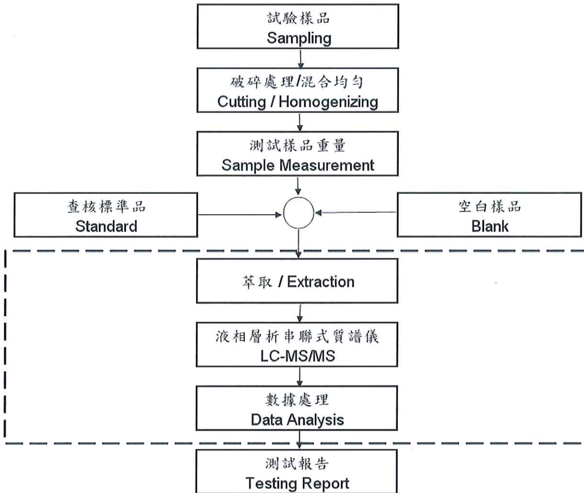
Flow Chart of Extraction for PFOS/PFOA
